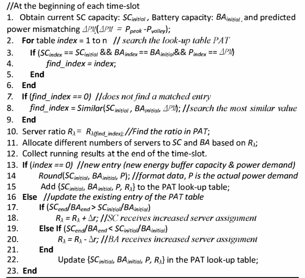
Figure 10. Algorithm for smartly handling large peaks
